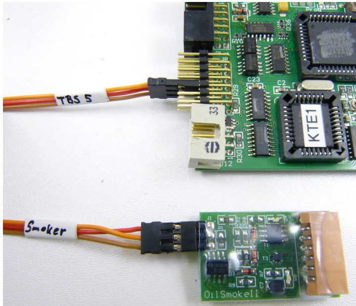
TBS5 Soundunit (3rd plug from bottom)
